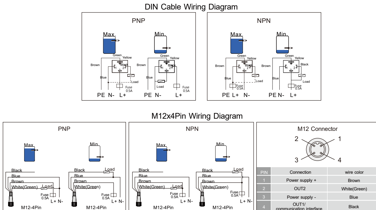
Figure 2 PNP / NPN Output Wiring Diagram
