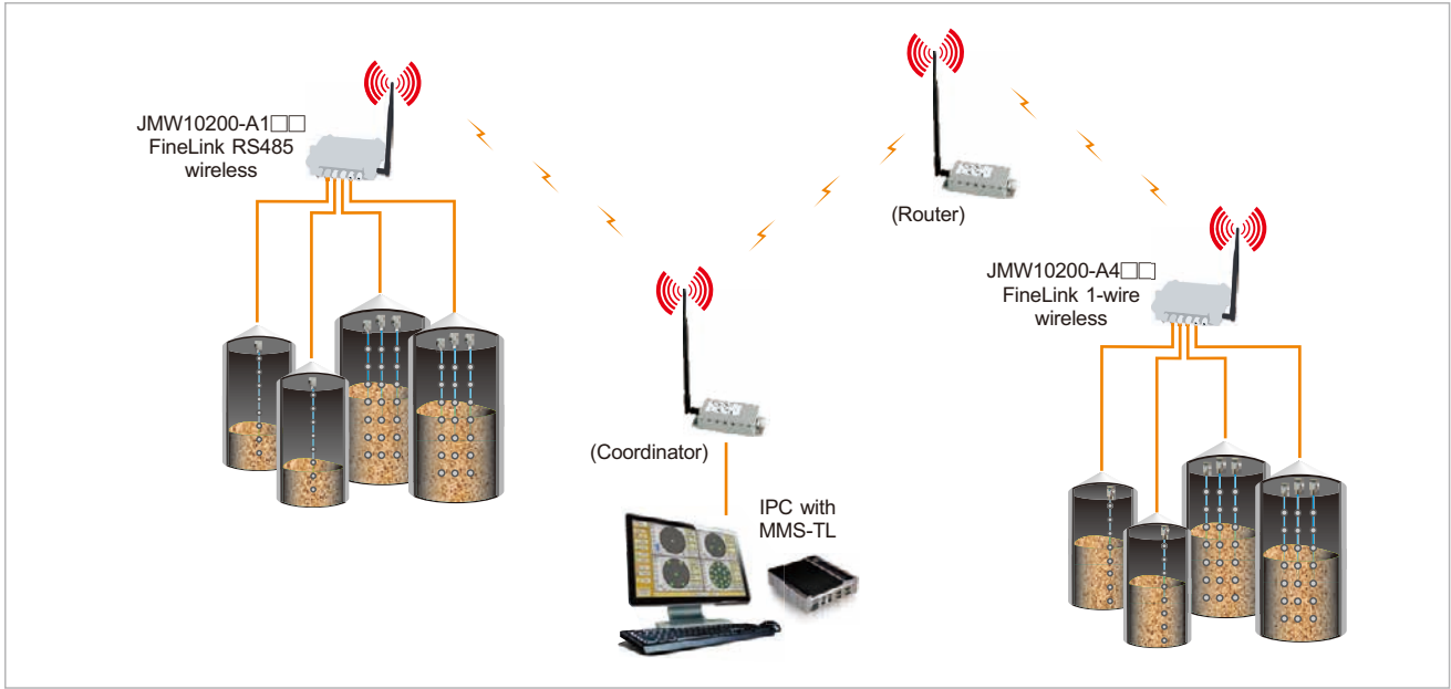
FineLink Wireless uses wireless to transmit RS485 signal, help customer reduce cable and maintenance costs.
