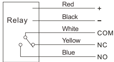
Fig. 8, 5A Relay output type wiring
