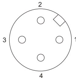
Fig. 12 Terminal diagram (NPN & PNP and 1A Relay output type)
