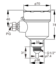
Fig. 15 SP210 5A(Relay)
