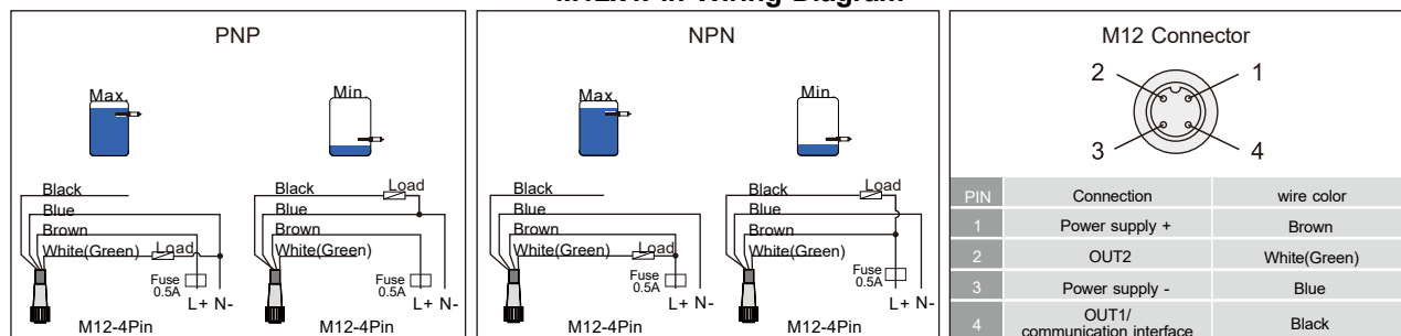
Figure 2 PNP / NPN Output Wiring Diagram
